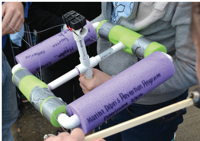
Marine Debris Tracking GPS Device
